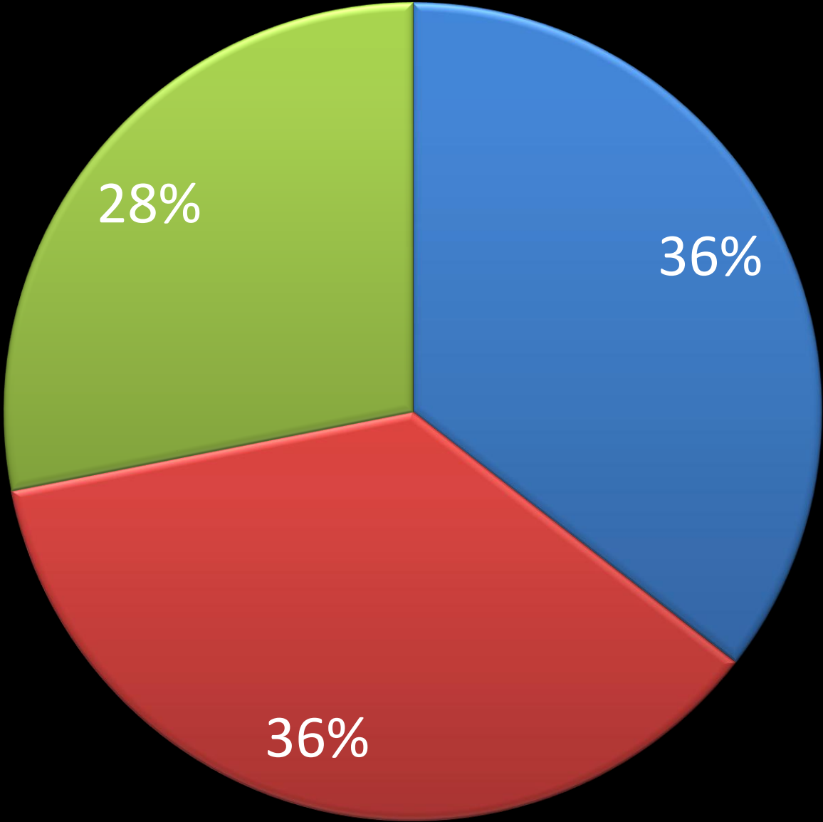
Percent Composition of a mixture containing sand, salt, and iron
